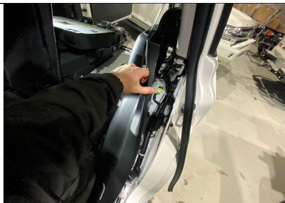
STEP 1.19 MOVE TO THE SECOND ROW PASSENGER DOOR AND BEGIN PULLING BACK QUARTER PANEL AGAIN CHECKING TRIM CLIPS.
